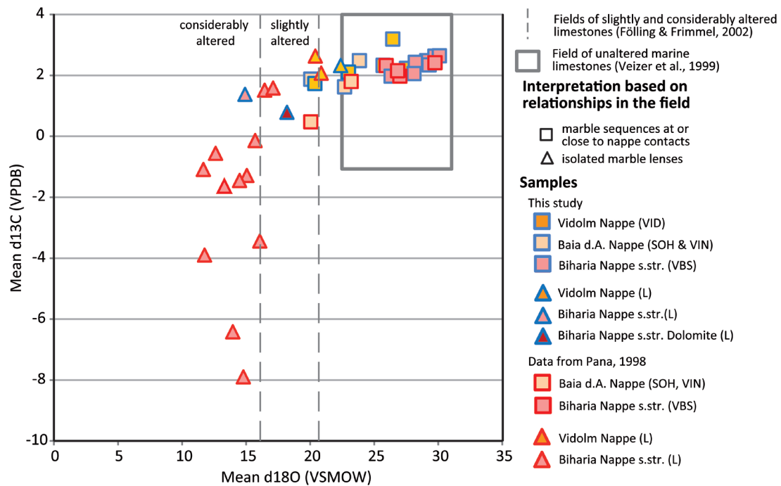
Fig. 7. Plotted results of the data from \delta^{18}\text{O} and \delta^{13}\text{C} isotope analyses. Data from the present study and data from Pană (1998) are discriminated by a red frame.
