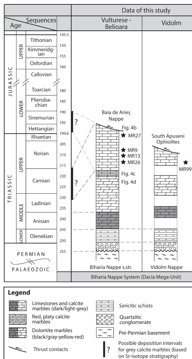
Fig. 9. Stratigraphic columns to allow for a tentative correlation of the sedimentary sequences of the Biharia Nappe System. Dashed lines indicate tentative correlations between the lithostratigraphic units. For the Vidolm occurrences, only the relative succession is given in the figure.
