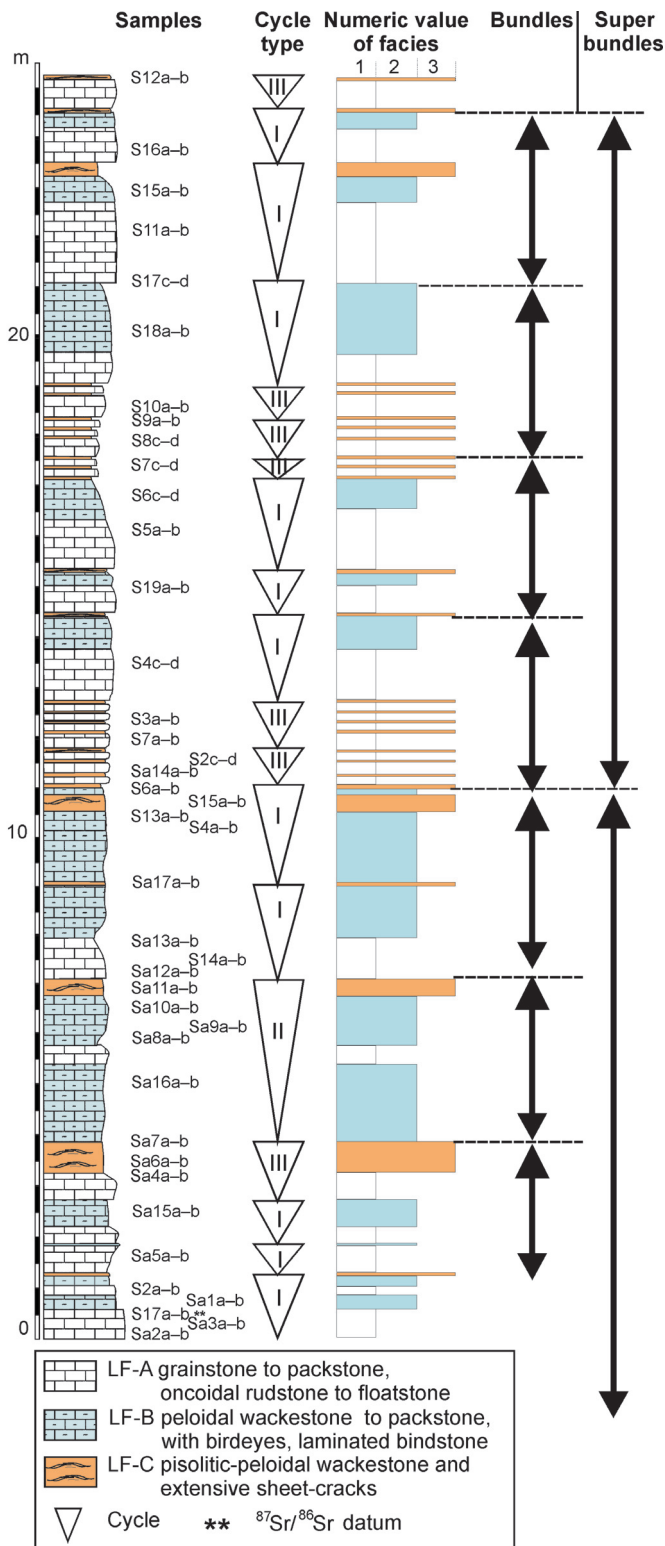
Fig. 2. Measured section from the Calcare Massiccio Formation and thickness recurrences of the main facies associations.
