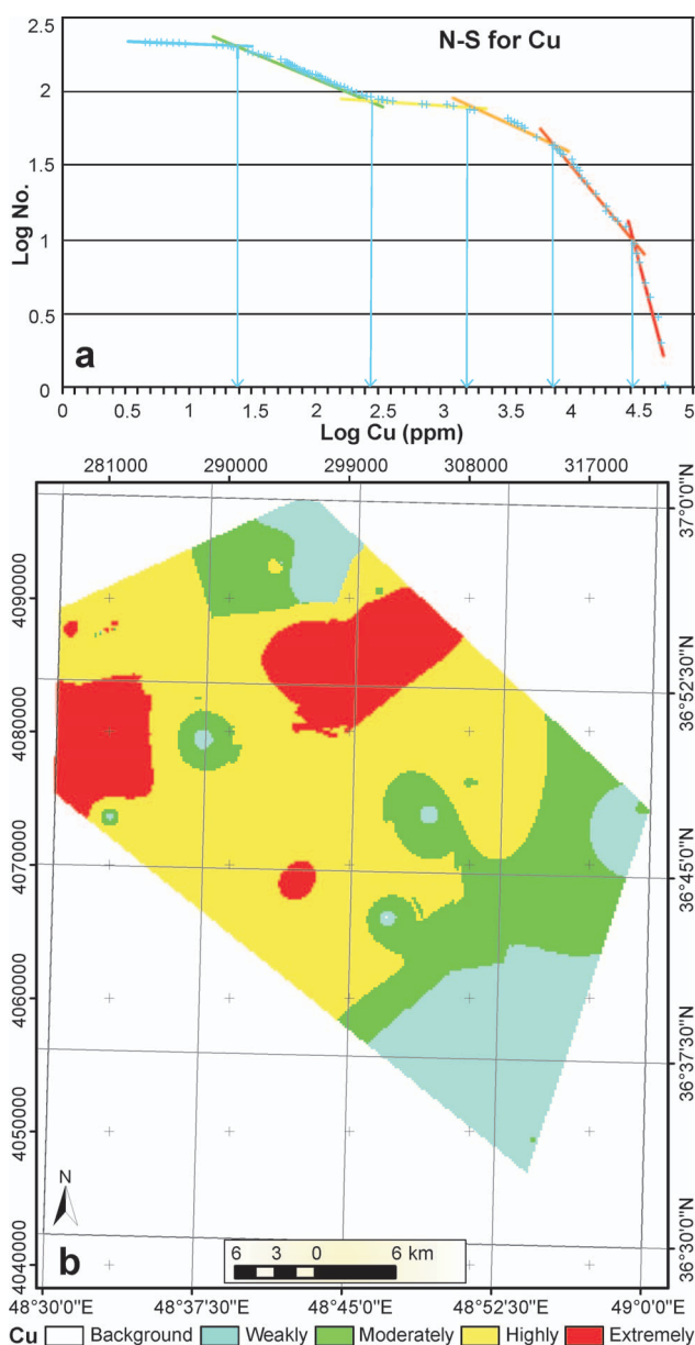
Fig. 5. a — Log-log plot of N-S method for Cu lithochemical data. b — Cu lithochemical population distribution map based on the N-S model.
