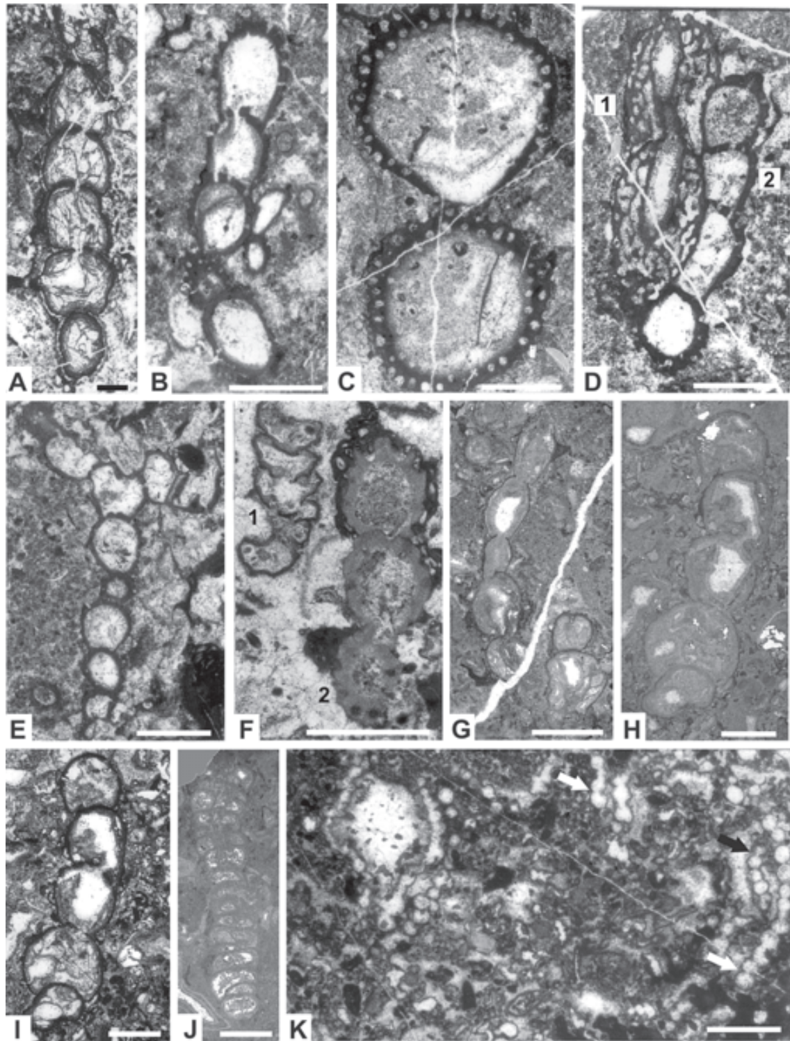
Fig. 4. Text continues from the previous page. ... Colospongia is missing and the three chambers are lying on the first chamber wall of Solenolmia . Despite this the wall of the fourth chamber of Colospongia is well developed and here Solenolmia has no wall. E — Colospongia catenulata catenulata Ott. Longitudinal section through a branched specimen shows the uneven perforation of the chamber walls (Fig. 7). 79/4/1. F — 1 — Chambered sponge? or foraminifer? gen. et sp. indet. and 2 — Colospongia catenulata catenulata Ott. 79/2a. G — Follicatena cautica Ott. Sections through two specimens show similar characteristics as Fig. A. 79/3b. H — Follicatena cautica Ott. Longitudinal section similar to Fig. A. 79/2/2a. I — Follicatena cautica Ott. Longitudinal section similar to Fig. A. 79/2/2a. J — Amblysiphonella sp. Longitudinal section through numerous low rectangular to crescent-shaped chambers. In the upper part of the sponge the spongocoels are cut. 79/17/1b. K — Olangocoelia otti Bechstäd & Brandner. Section through numerous small spherical chambers arranged in rows. Chambers are connected either directly or by a short and narrow tube (arrows). 79/51.
