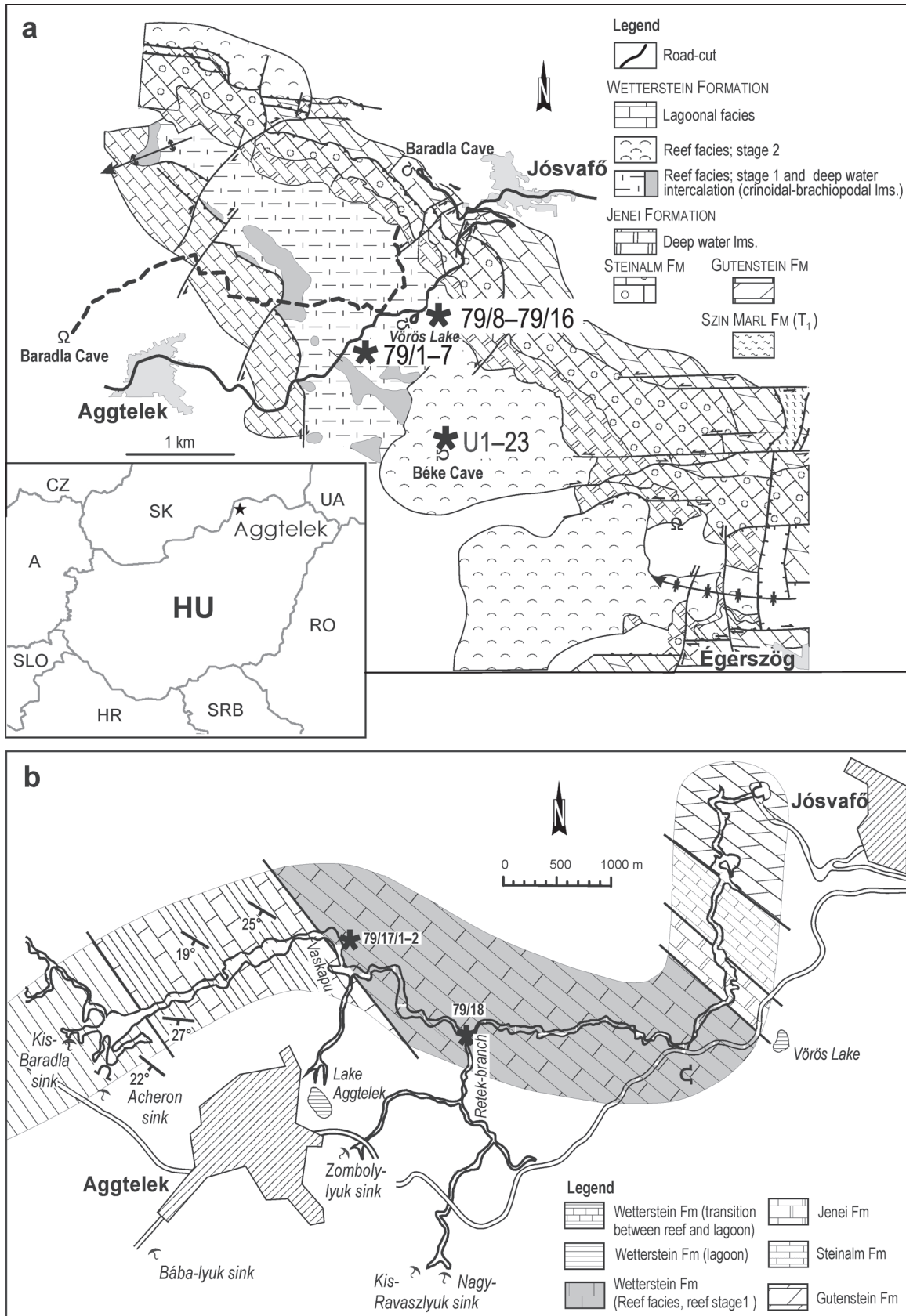
Fig. 1. a — Geological map of the Aggtelek-Jósvafő area (Velledits et al. 2011) and the sampling points (asterisks). Dashed line depicts the vertical projection of the Baradla Cave. Asterisks — locations of the samples from surface exposures. b — Middle Triassic formations revealed by the Baradla Cave with the location of the sampling points.
