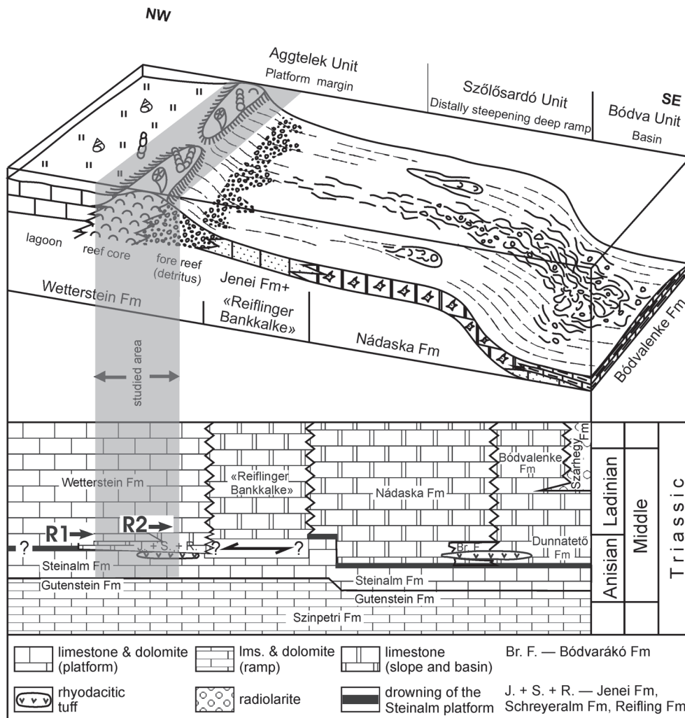
Fig. 2. Middle Triassic depositional model and Triassic lithostratigraphy of the Aggtelek and neighbouring units. (Modified after Kovács 1997.) Light grey shading indicates the studied area. R1 — Wetterstein Formation reef facies, stage 1. R2 — Wetterstein Formation reef facies, stage 2.
