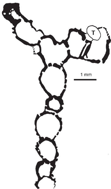
Fig. 7. A branched specimen of Colospongia catenulata catenulata Ott shows the unevenly distributed pores of the chamber walls. T — A specimen of a “ Tubiphytes ”-like organism embedded in the chamber of the sponge (drawn from Fig. 4E).
