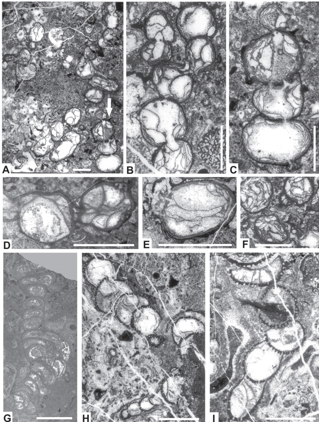
Fig. 6. “Sphinctozoans” from the Anisian-Ladian Aggtelek reef limestones, NE part of Hungary. Scale in all figs. 5 mm. A–F — Follicatena cautica Ott. A — Several longitudinal, oblique and cross-sections showing the abundance of sponges in the investigated material. For magnification of the specimen indicated with an arrow see Fig. C. 79/3c. B — Section through a branched specimen showing the single openings or sieve-plates in the chamber walls and the vesiculae within the chamber interiors. U3a. C — The magnification from Fig. A (white arrow) shows four chambers with thin walls, the perforation pattern of chamber walls and the abundance of concentric vesiculae within the chambers. 79/3c. D — Section through two chambers showing the vesiculae within the chamber interiors and the sieve-plates in the chamber walls. U16. E — Similar to Fig. D. The sieve-plate with several openings is clearly visible. U8c. F — Cross-sections through three chambers showing the abundant vesiculae within the chamber interiors. 79/3b. G — Amblysiphonella sp. The specimen seems to be branched in the middle part or the ‘normal’ growth has been interrupted. 79/17/1a. H — Colospongia catenulata macrocatenulata Scholz. Section through two specimens (or a branched specimen?) with numerous spherical chambers. Chamber walls are pierced by evenly distributed pores. Some vesiculae are within the chamber interiors. 79/9a. I — Colospongia catenulata macrocatenulata Scholz. Section through a specimen showing similar characteristics to the sponge in Fig. H. 79/9b.
