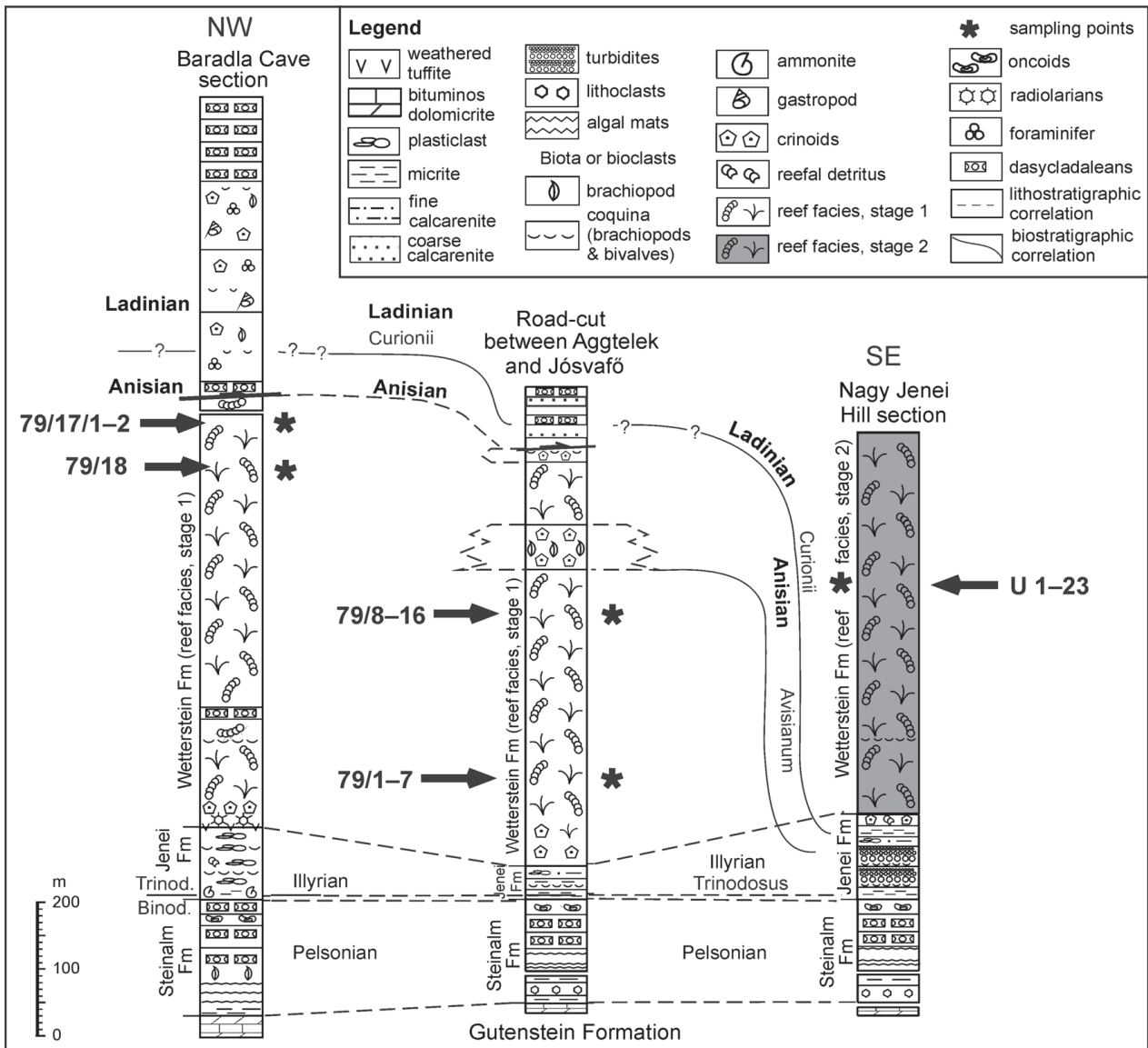
Fig. 3. Stratigraphical positions of the samples.
