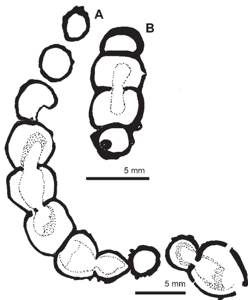
Fig. 11. Kovacsia baloghi (Kovács). A — The holotype of the species drawn from Kovács (1978a: fig. 6C) and B — from Fig. 9E (this paper). Both species show the thin spongocoel wall followed the chamber exowalls. The holotype shows two openings in one chamber roof and only one opening in three chamber roofs. Rarely ostia are cut in the chamber exowalls of both specimens.
