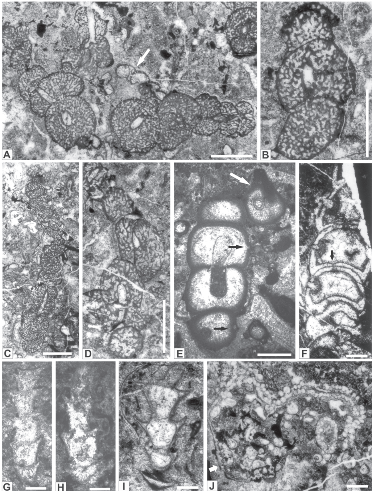
Fig. 9. “Sphinctozoans” from the Anisian-Ladian Aggtelek reef limestones, NE part of Hungary. Scale in A–D = 5 mm, in E–F and J = 2 mm, in G–I = 1 mm. A–D — Solenolmia manon manon (Münster). A — Longitudinal and oblique sections through several specimens showing the spherical to hemispherical chambers with thin chamber walls and reticulate filling skeleton within the chamber interiors. The axial spongocoel is about 1/5 of the whole sponge diameter. The arrow indicates a specimen of Colospongia catenulata catenulata Ott. 79/14b. B — Oblique section through three chambers clearly exhibiting the reticulate filling skeleton and the thin chamber walls. 79/14a. C — Marginally... Continues on the next page
