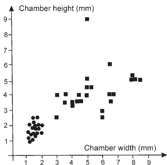
Fig. 5. Ratio of chamber height/chamber width in Colospongia catenulata catenulata Ott (dots, 19 measurements) and Colospongia catenulata macrocatenulata Scholz (rectangle, 24 measurements).
