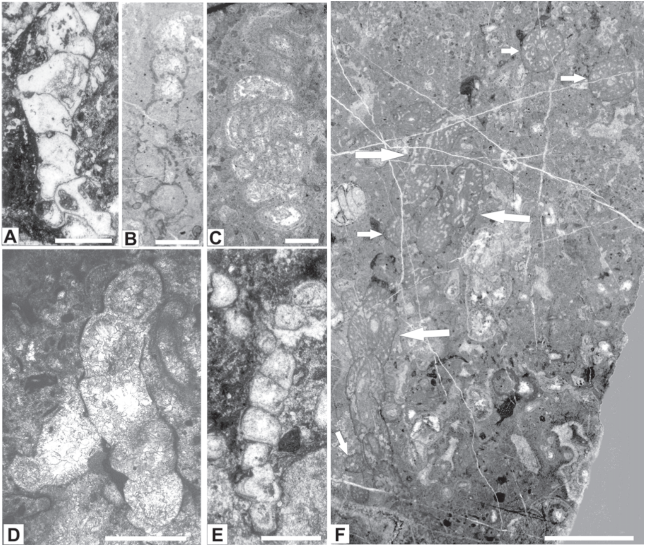
Fig. 8. “Sphinctozoans” from the Anisian-Ladian Aggtelek reef limestones, NE part of Hungary. Scale in all figs. 5 mm. A — Celyphia? sp. Longitudinal section through several irregularly arranged chambers with thin chamber walls. 79/51. B — Colospongia catenulata catenulata Ott. Longitudinal section through numerous spherical chambers with evenly perforated chamber walls. 79/3b/2. C — Amblysiphonella sp. Longitudinal section through several rectangular chambers. The section exhibits in the middle part the existence of one (or several?) spongocoel(s). 79/17/1a. D — Celyphia zoldana Ott, Pisa & Farabegoli. Section through several circular to rectangular chambers. U8c. E — Celyphia zoldana Ott, Pisa & Farabegoli. Similar to Fig. D. 79/17/2b. F — Solenolmia radiata Senowbari-Daryan & Riedel. Cross (small arrows) and longitudinal sections (large arrows) through several specimens. U9c.
